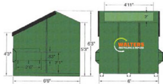
8 YARD FR. SLANT DOCK
