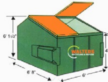
8 YARD SLANT
