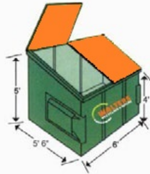
4 YARD
