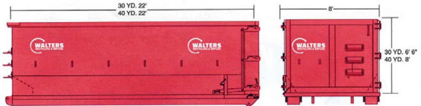
30 & 40 YARD OPEN TOP
