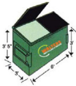
2 YARD
