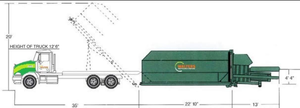
ROLL OFF VEHICLE CONFIGURATION
