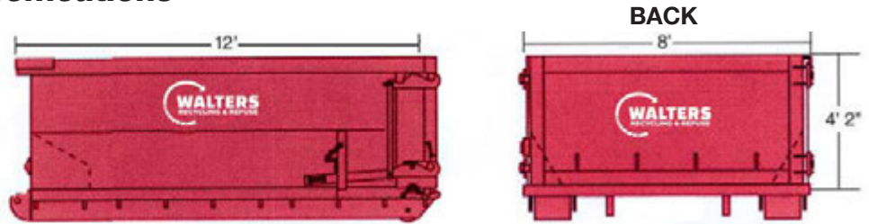
10 YARD OPEN TOP
